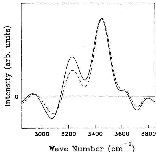
FIG. 3. Raman spectra from Fig. 2 after Fourier deconvolution for 22 (full line) and 24 °C (dashed line). The spectra are normalized so that the lines about 3450 \text{cm}^{-1} are of equal height.
